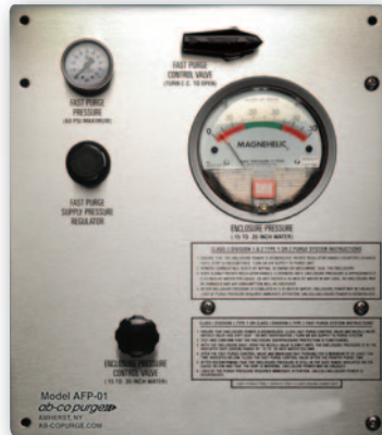
AFP-01Z-15 Z Purge Unit Up to 15 cu. ft.
